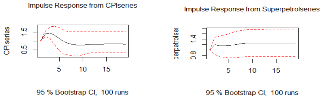
Figure 16. Impulse Response of CPI to CPI and Petrol to Petrol
