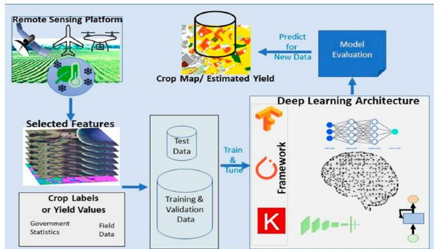
Figure 1. Overview of Deep-Learning Architectures in Agricultural Modeling
