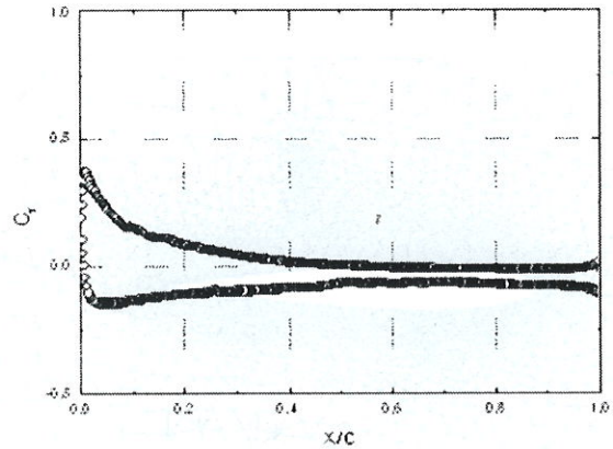
Figure 7: Skin-friction distribution for a viscous-flow ( M_x = 0.80 ), ( \alpha = 10^\circ ) and ( Re_x = 500 )
