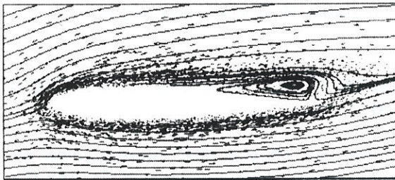
Figure 5: Laminar viscous flow around NACA0012 airfoil. Streamlines in the separation region ( M_x = 0.80 ), ( \alpha = 10^\circ ) and ( Re_x = 500 )
