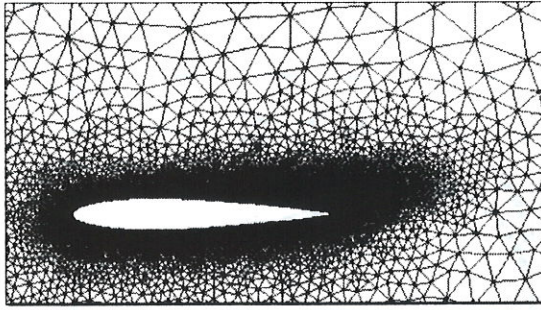
Figure 4: Close-up of regenerated mesh, Viscous-flow ( M_x = 0.80 ), ( \alpha = 10^\circ ) and ( Re_x = 500 )
