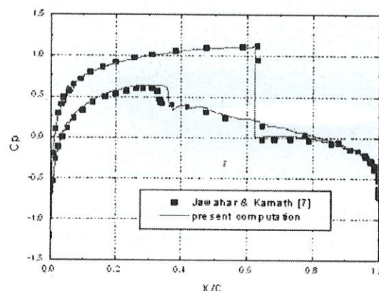
Figure 3: Surface pressure distribution for NACA 0012 transonic flow, ( M_\infty = 0.80 ) and ( \alpha = 1.25^\circ )
