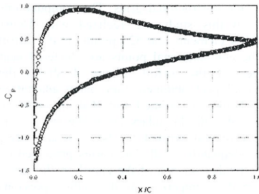
Figure 6: Pressure distribution, Viscous-flow, ( M_x = 0.80 ), ( \alpha = 10^\circ ) and ( Re_x = 500 )
