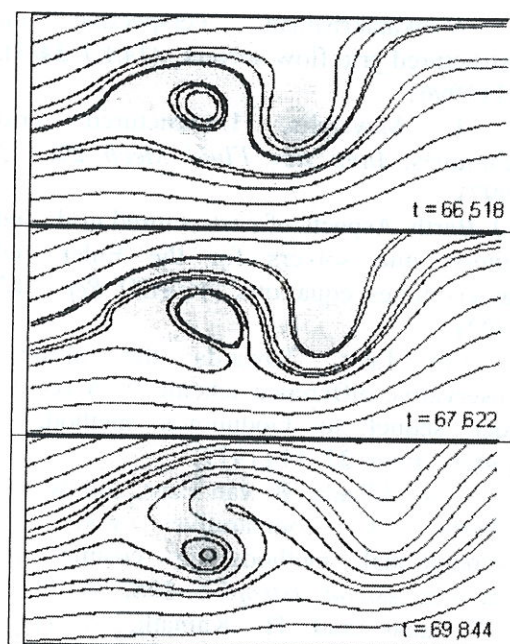
Figure 9: Instantaneous stream lines NACA0012, ( Re = 22000 , Mach = 0.1 and angle of attack = 30^\circ ) (Times are in seconds).
