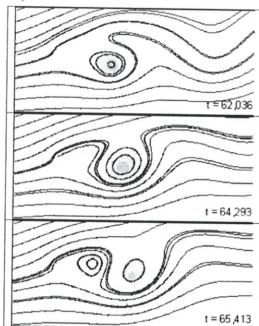
Figure 8: Instantaneous Mach number contours NACA0012, ( Re = 22000 , Mach = 0.1 and angle of attack = 30^\circ ) (Times are in seconds).
