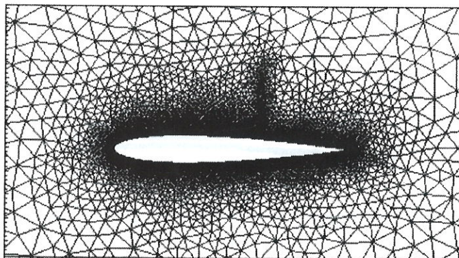
Figure 1: Close-up of adaptive meshes for NACA 0012 airfoil at ( M_\infty = 0.80 ) and ( \alpha = 1.25^\circ ).
