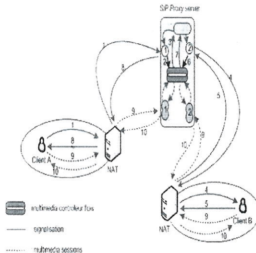
Fig.13. Call establishment
