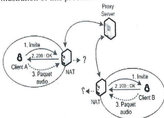
Fig. 8. NAT and media stream
