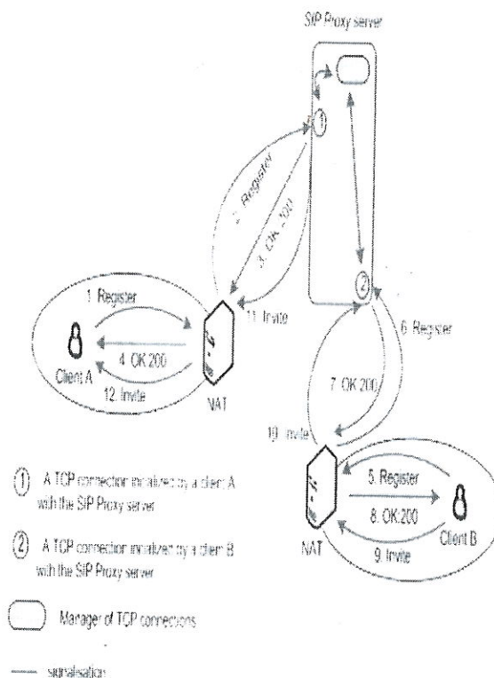
Fig.11. The adaptation of TURN in signalling phase
