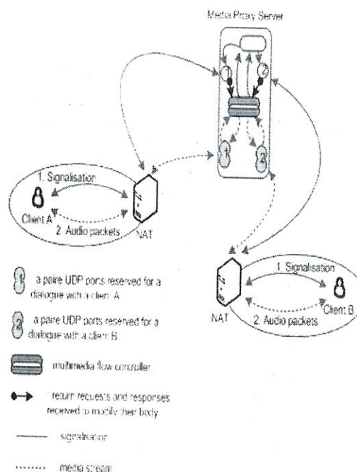
Fig.12. The adaptation of TURN in media stream phase
