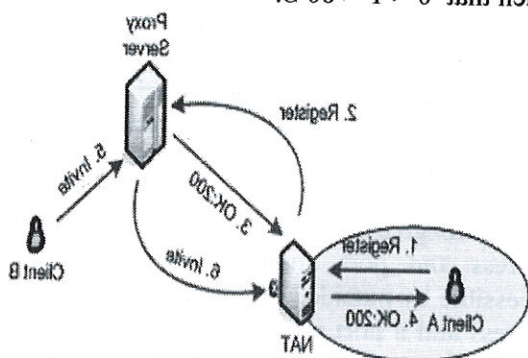
Fig. 7. Signalisation and NAT
