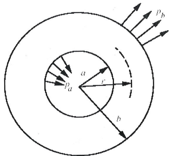
Figure 10: A hollow circular cylinder with pressure applied on the inner and outer surfaces.
