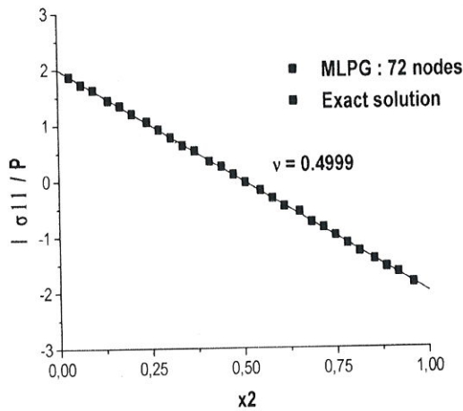
Figure 7b: \sigma_{11} vs. x^1 on the top
