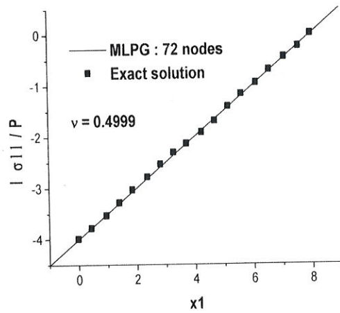
Figure 7c: \sigma_{11} vs. x^2 at x^1 = 4
