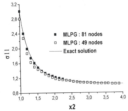
Figure 9: \sigma_{11} vs. x^2 at x^1 = 0 .
