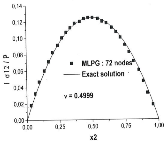
Figure 7d: \sigma_{12} vs. x^2 at x^1 = 4
