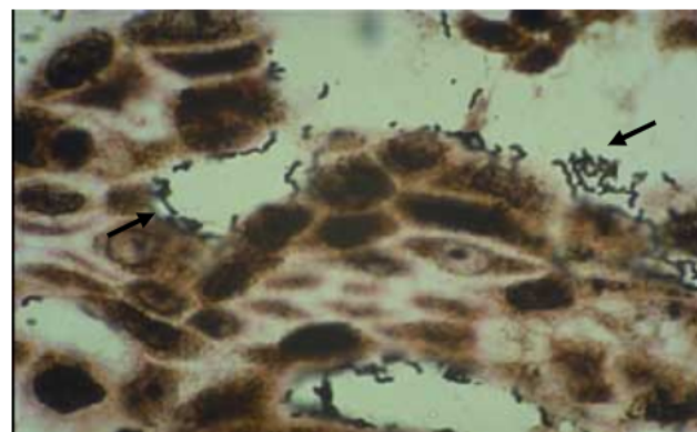
Figure 1: Examination anatomopathology of biopsic gastric by the technique of colouring of "Warthin Starry ", indicating the presence of H. pylori
