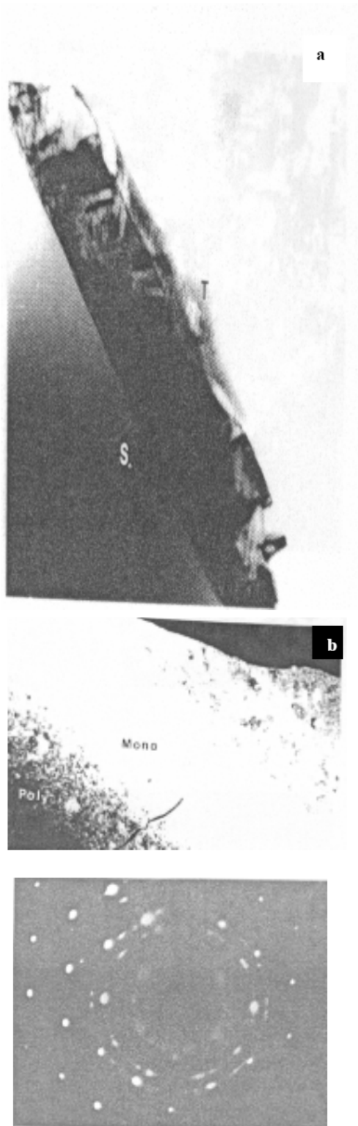
Fig.6 : a) Cross-section of the 1000 Å amorphous Si layer irradiated by 3 shots of YAG laser ( 2 \text{ J/cm}^2 ) b) alternated poly and monocrystalline regions c) associated diffraction pattern
