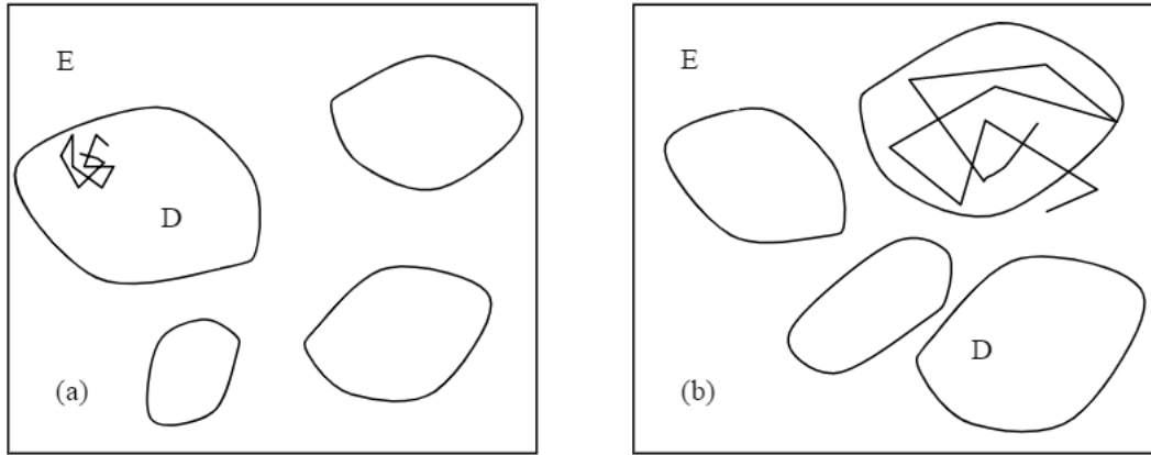
Figure 6: Qualitatively, we represent the space of polynomials (E) and the domains (D), non convex, in solid curve, the regions where the polynomials are orthogonal. The round off error in computation generate a random walk in this space (broken line). When the size of the network is small the random walk has little steps (a), when the size of the network is large big steps (b).
