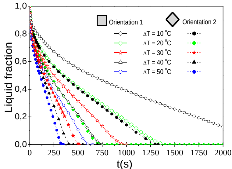
Fig. 8. Variations of liquid fraction with time at different temperature differences in solidification case.
