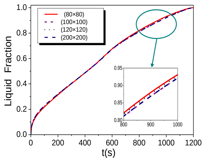
Fig. 3. Effects of grid size
