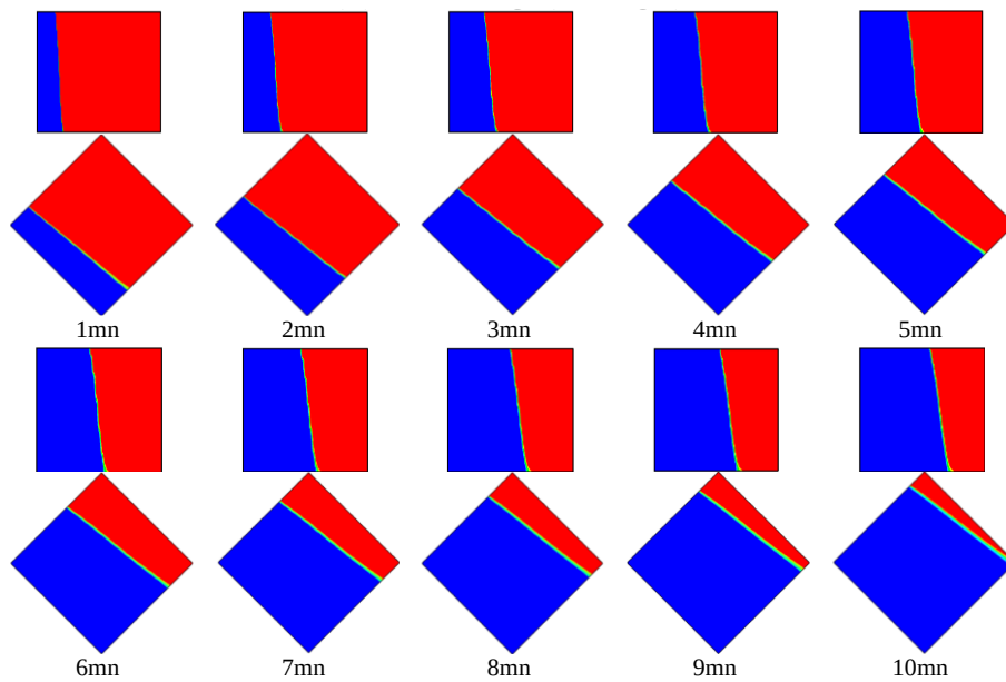
(b) Solidification (discharge) process,
