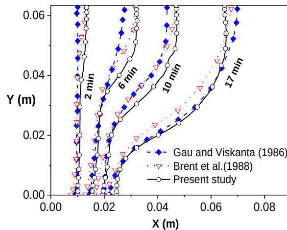
Fig. 4. Comparison of melting front at various times obtained by the present study and previously reported works.
