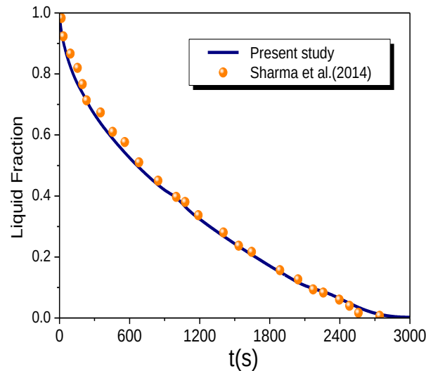
Fig. 5. Comparison of volume fraction profile from solidification between the present study and those of Sharma et al. [24].
