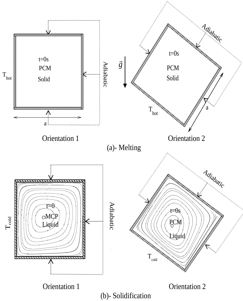
Fig. 1. Physical model and boundary conditions
