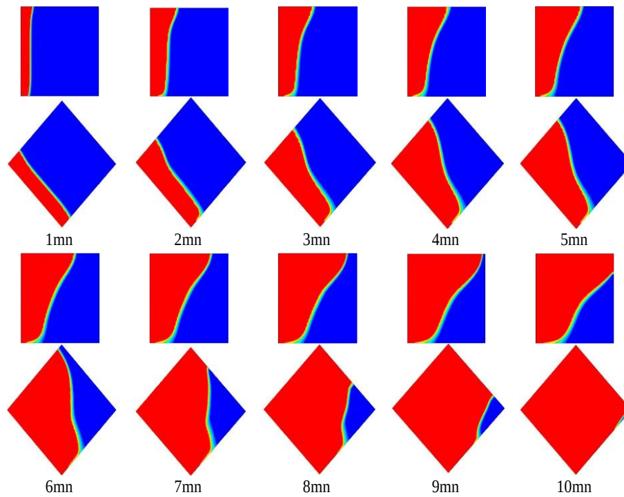
(a) Melting (charge) process
