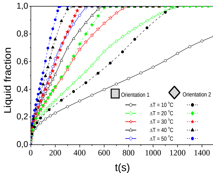
Fig. 7. Variations of liquid fraction with time at different temperature differences in melting case.
