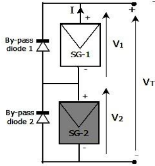
Fig. 3: Configuration of the module into two subgroups of 18 cells each
