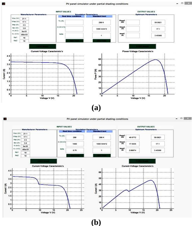
Fig. 5: Curves for standard test (a) and 25% shaded PV panel (b)
