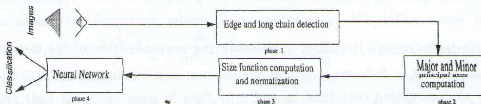
Figure 5: Recognition System Architecture
