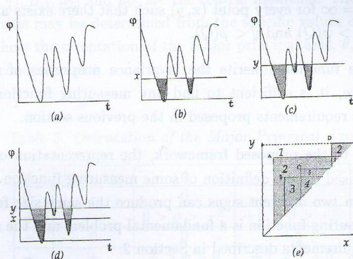
Figure 2: Example of a size function. (a) Graph of some measuring function \varphi . (b) and (c) The shaded regions identify the sets of points with \varphi \leq x and \varphi \leq y respectively. (d) The darker shading identifies the regions with both \varphi \leq x and \varphi \leq y . (e) Graph of the size function l_\varphi(x, y) for all possible values of x and y . Each label denotes the value of l_\varphi within the underlying region.
