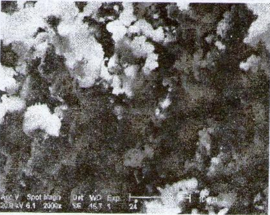
Fig.3. Scanning electron micrograph of TiAl alloy powder after reduction by calcium at 1247 K during 7.2 Ks and milling during 1.8 Ks
