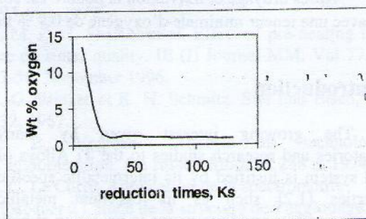
Fig.2. Influence of reduction time on oxygen residual content
