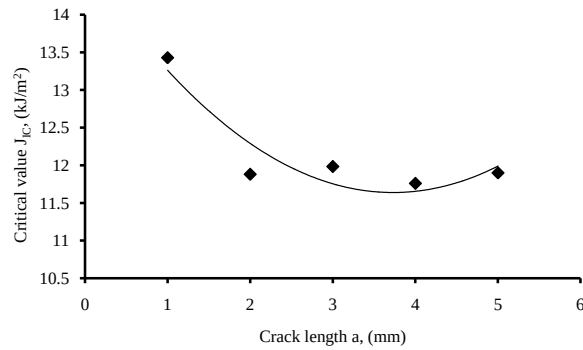
Figure 7. Variation of J_{IC} vs crack length a
