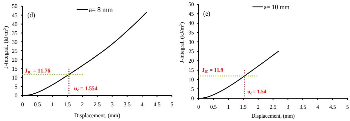
Figure 6. Variation of fracture toughness J_{IC} vs displacement for different crack length
