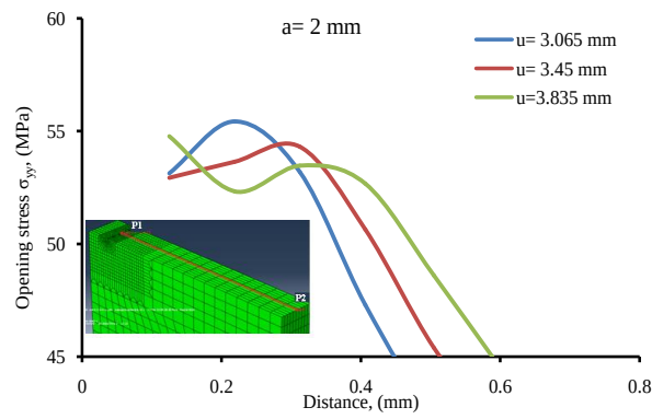
Figure 5. Opening stress ( \sigma_{yy} ) distribution along the crack line of the ligament (P1-P2), notch of 2mm
