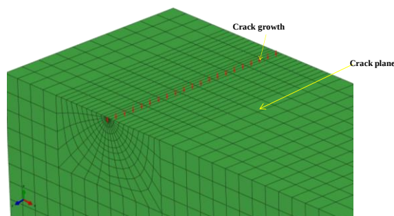
Figure 3. Crack growth direction
