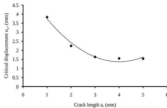
Figure 8. Variation of u_c vs crack length a
