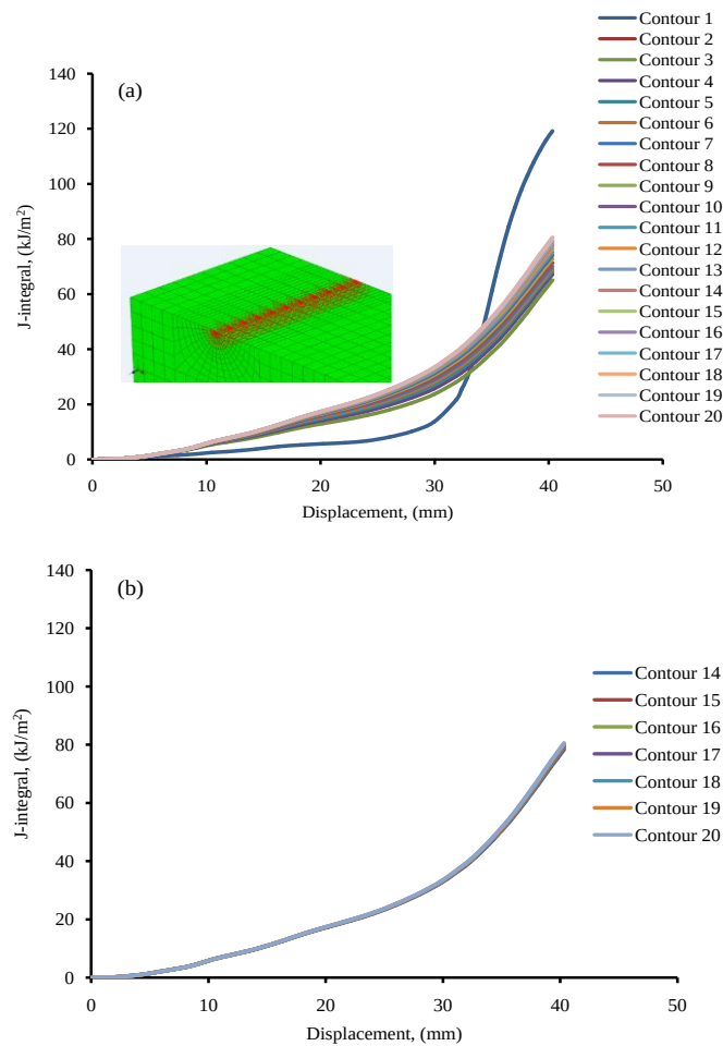
Figure 4. Evolution of the J-integral
