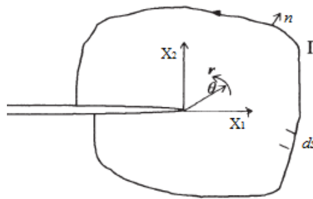
Figure 1. Path for the calculation of J-integral
