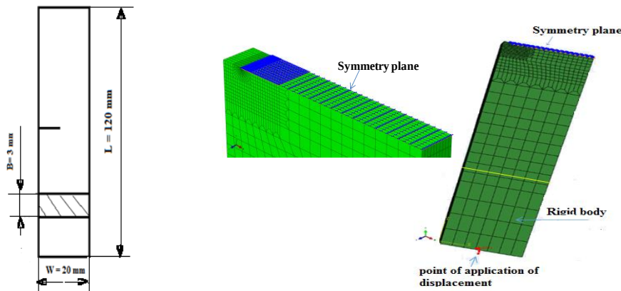
Figure 2. Specimen geometry, dimensions and 3D SENT model
