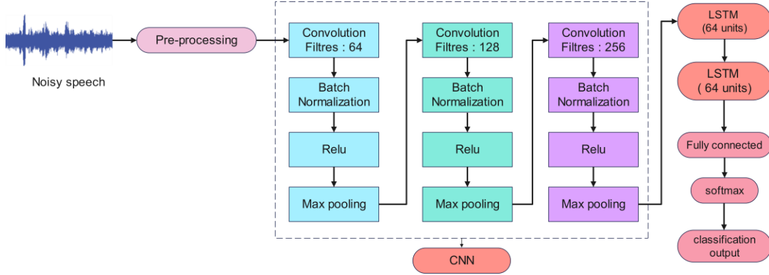
Figure 1. The proposed CNN-LSTM architecture for efficient ASR applied to noisy dataset.
