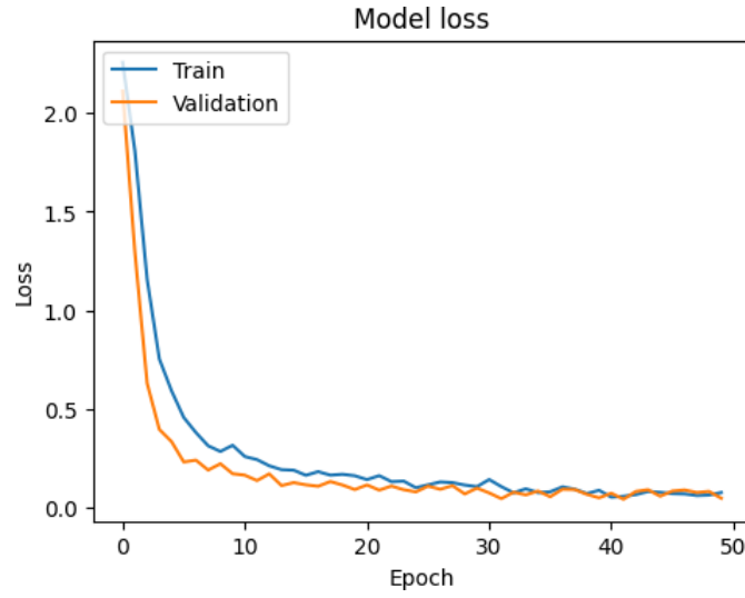
Figure 10. Model loss in clean speech (ASC-10 dataset).
