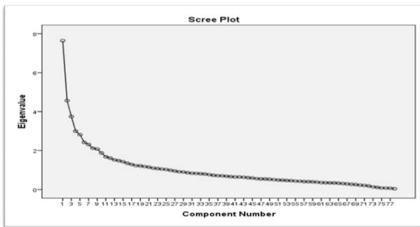
شكل 05: scree plot
