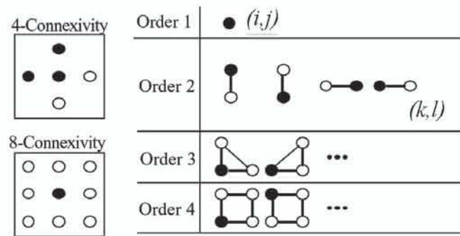
Fig 1. Neighbourhood and cliques
