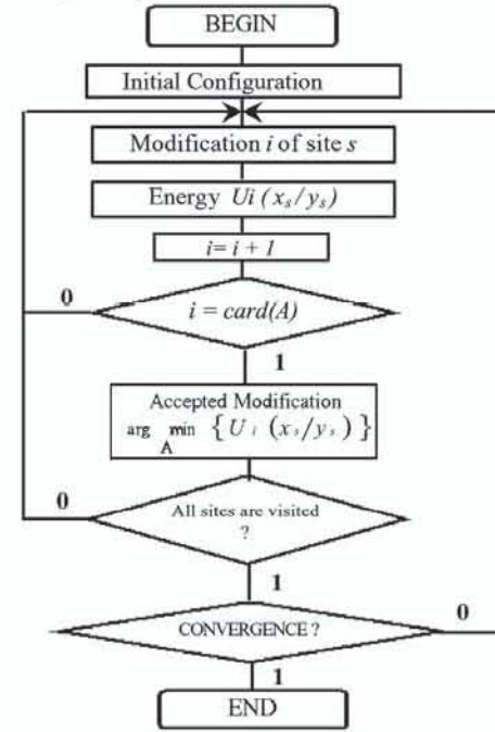
Fig 2. ICM flow chart
