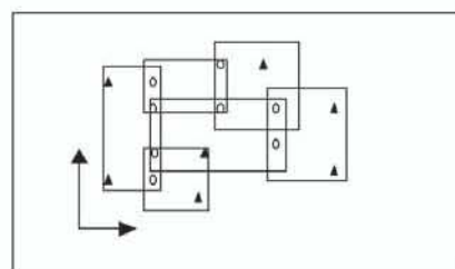
Fig. 3 : Example of repartition of planimetric controls, ties points and overlap between sheets.
