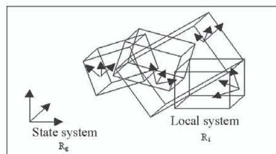
Fig. 2 : Local systems and state co-ordinates.
