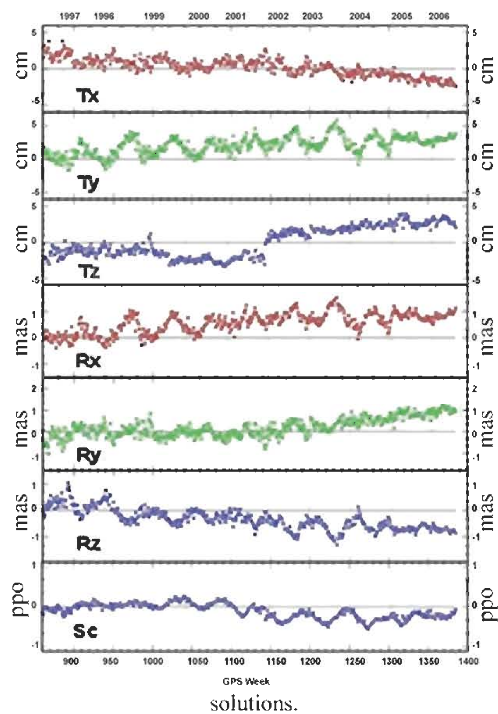
Fig. 2 The Helmert translation, rotation and scale parameters between the multiyear and the weekly solutions.
