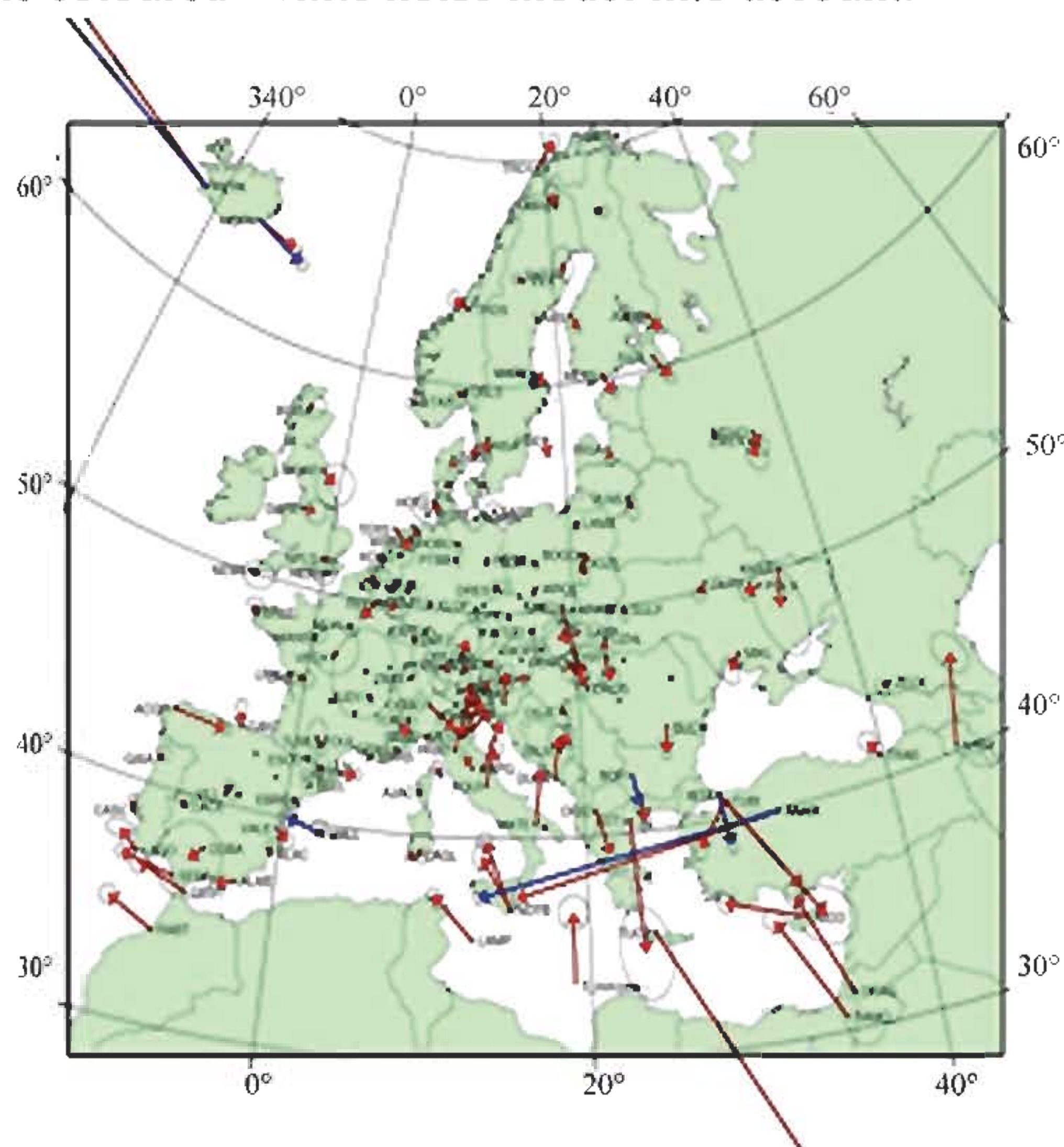
Fig. 8 The estimated EPN residual velocities wrt the Eurasian tectonic plate. Some sites have double velocity estimations, where following an event (equipment change, earthquake) the station had apparently different behaviour.
