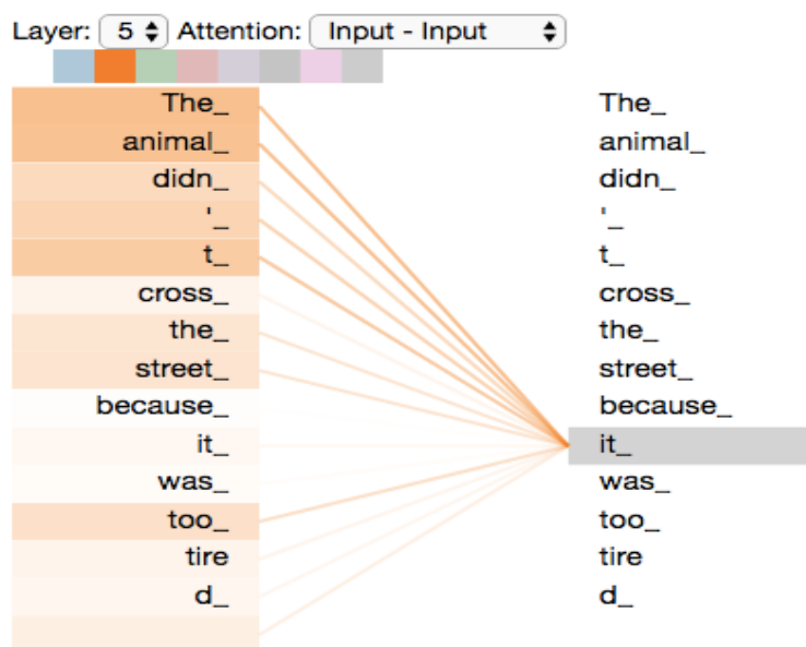
Figure 1. Self-attention at a high level. Reprinted from The Illustrated Transformer by J. Alammam (2018), retrieved from https://jalammam.github.io/illustrated-transformer/ ; licensed under CC BY-NC-SA 4.0
