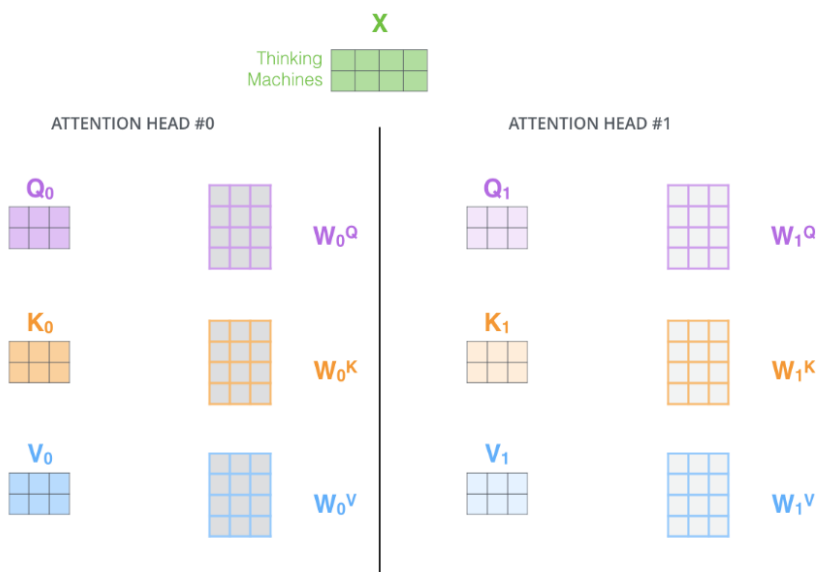
Figure 2. The beast with many heads (multi-headed attention). Reprinted from The Illustrated Transformer by J. Alammr (2018) https://jalammar.github.io/illustrated-transformer/ ; licensed under CC BY-NC-SA 4.0
